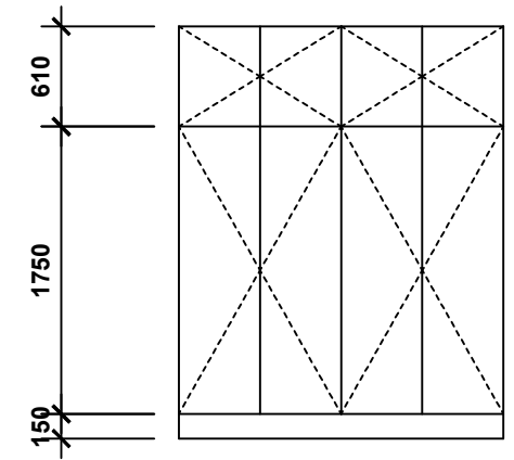
ELEVATION 4 scale 1:100
