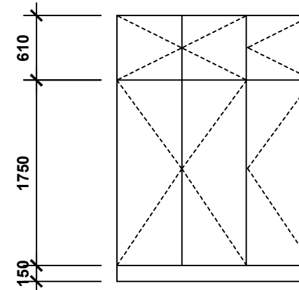
ELEVATION 5 scale 1:100
