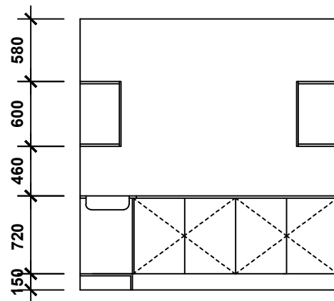
ELEVATION 8 scale 1:100
