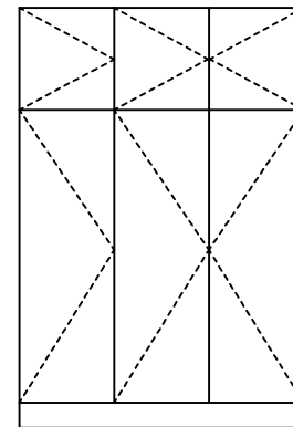
ELEVATION 6 scale 1:100
