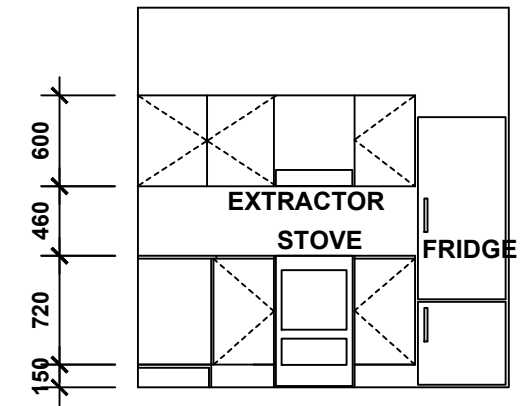
ELEVATION 12 scale 1:100
