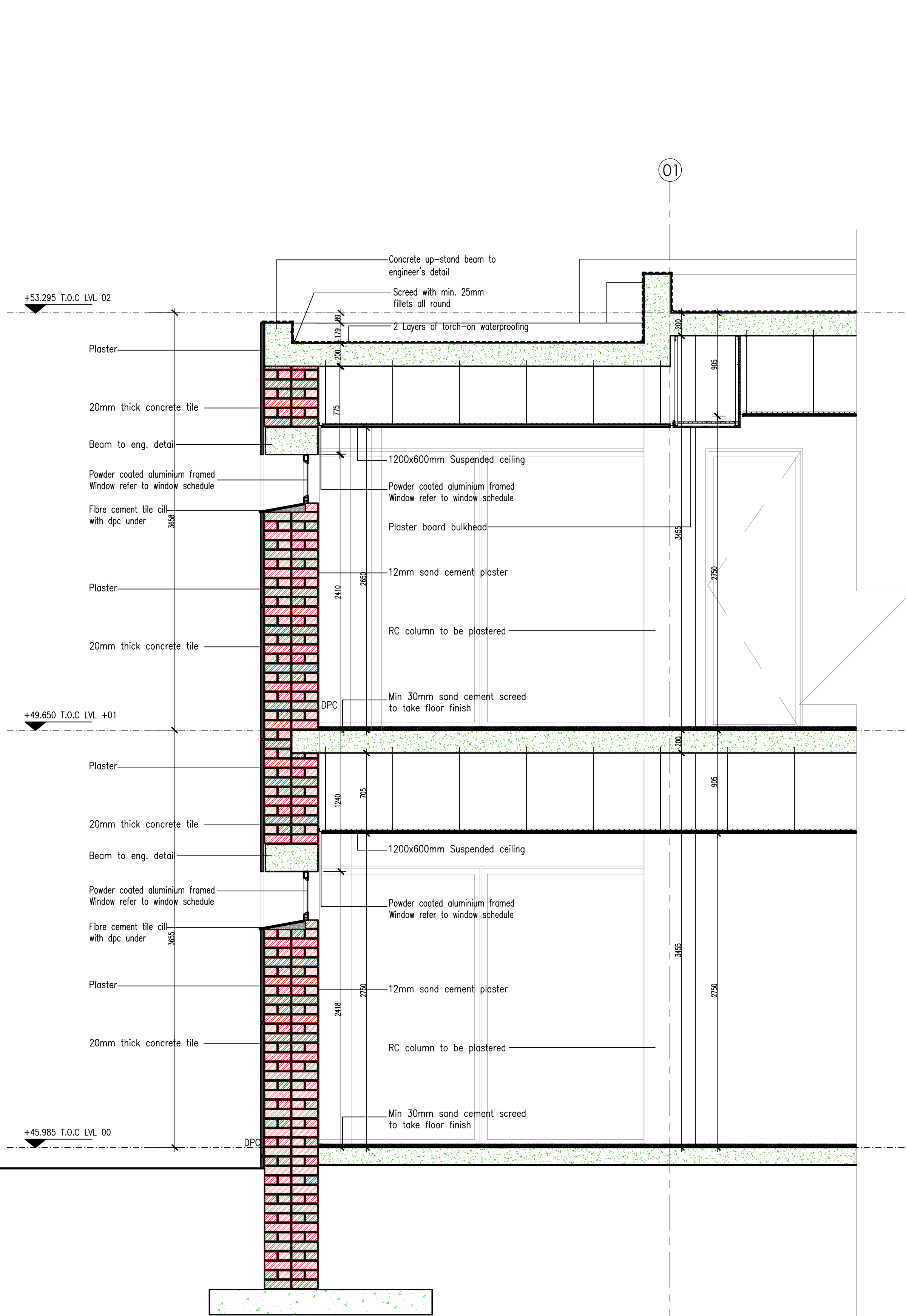
SECTION 07 SCALE 1:25
