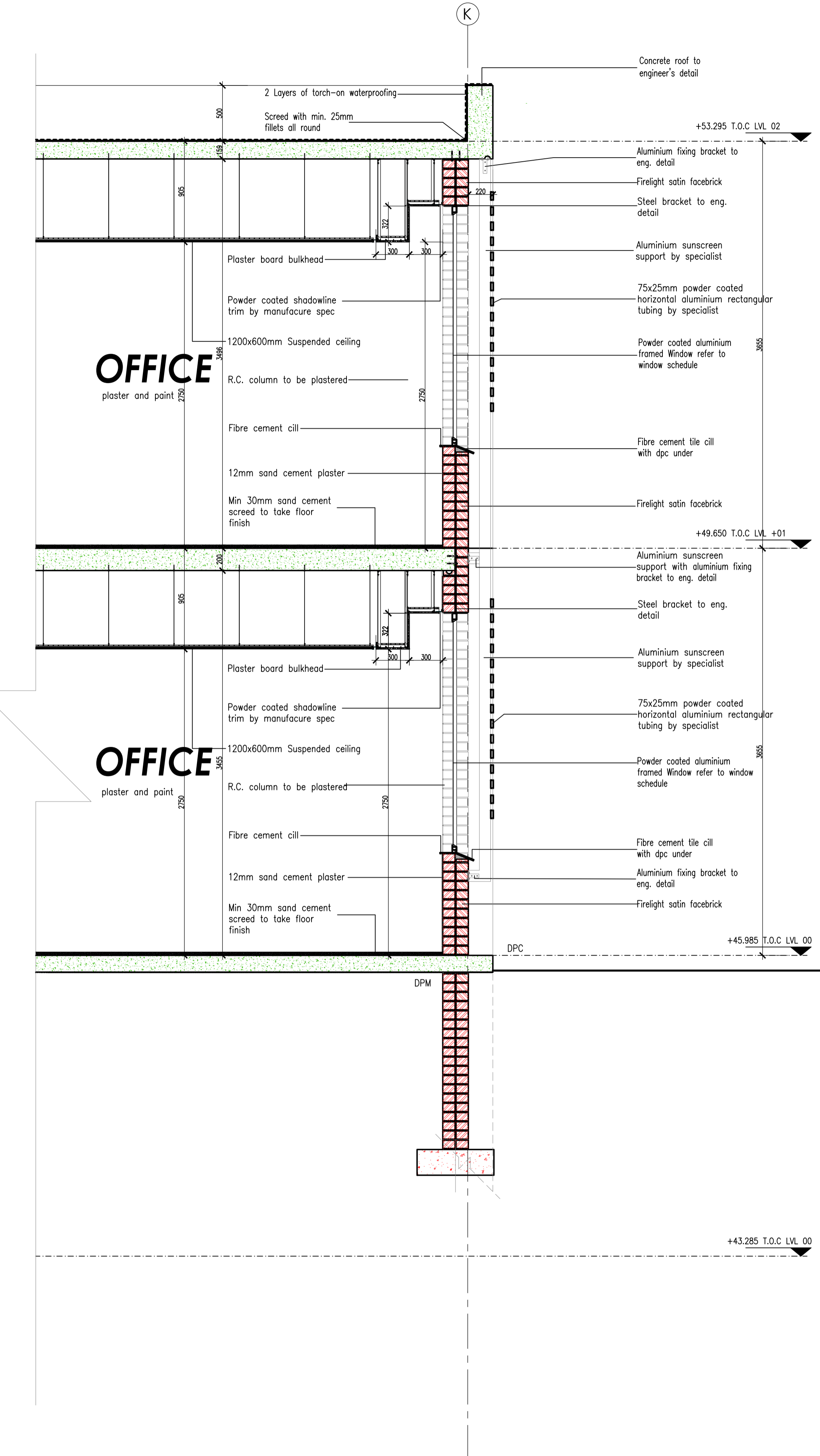
SECTION 02 SCALE 1:25
