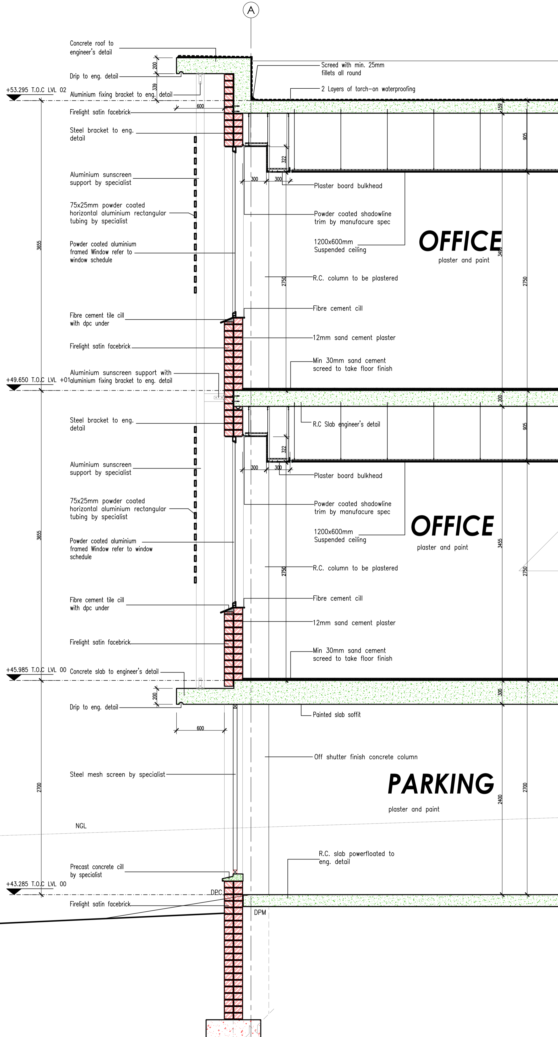
SECTION 01 SCALE 1:25
